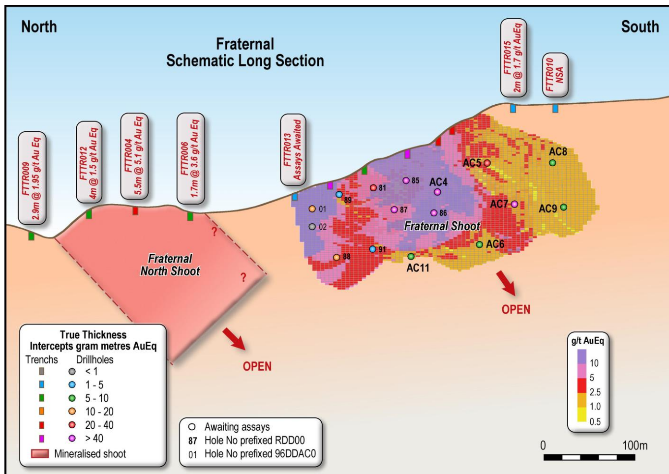
Figure 9. Long section with gold equivalent block model for the Fraternal Shoot.
