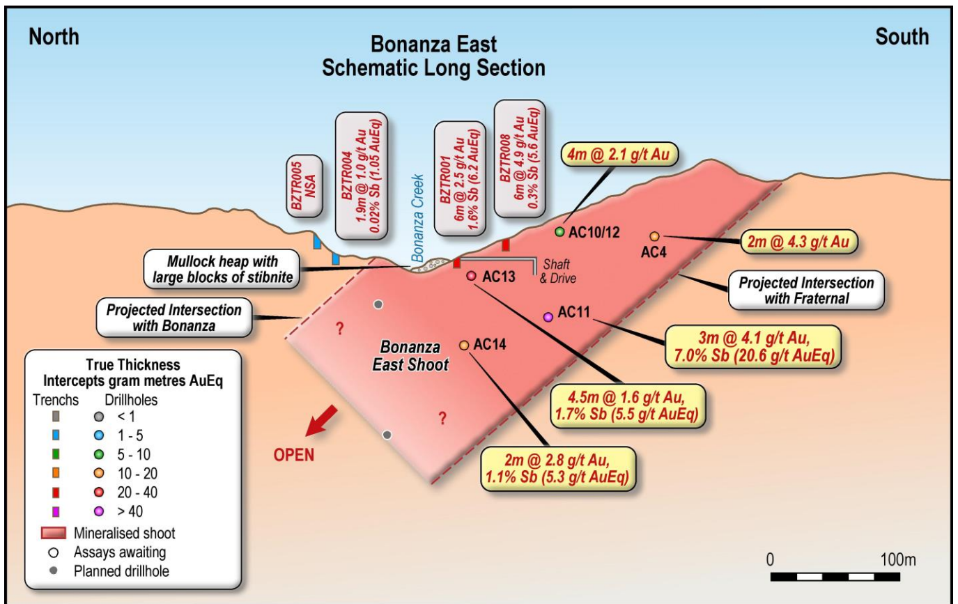
Figure 4. Bonanza East Shoot schematic long section.
