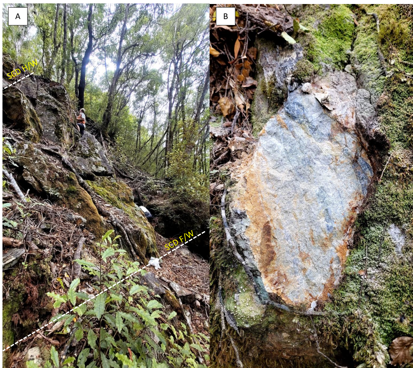
Figure 6. A. Outcrop of the SCD in the A2 Anticline at Doyles showing the hangingwall (H/W) and footwall (F/W). B. SCD footwall showing highly silicified and altered granite with arsenopyrite veinlets shown by dark grey. Rock chip assays obtained from this area have ranged from 1.0 to 9.6 g/t Au (refer table 2)
