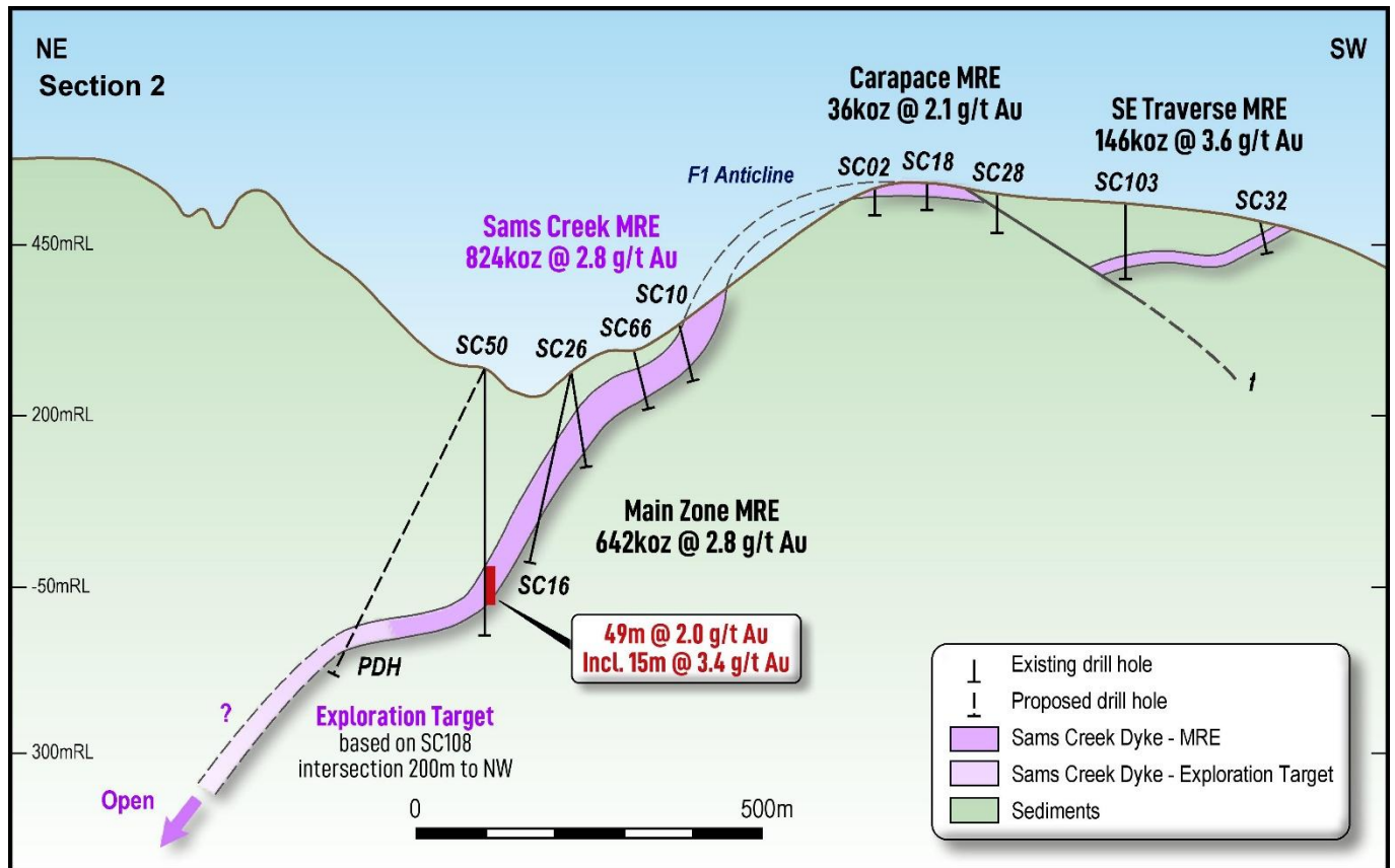
Figure 5. Schematic Cross-section 2 through the SE Traverse, Carapace and Main Zone mineralisation.
