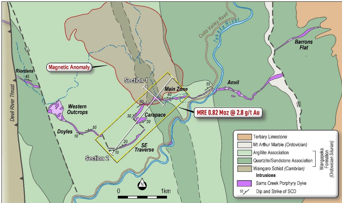
Figure 1: Geology of the Sams Creek deposit.
