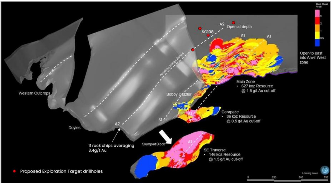
Figure 3: Plan view of undrilled SCD (grey) and MRE block model (magenta high grade, blue low grade).
