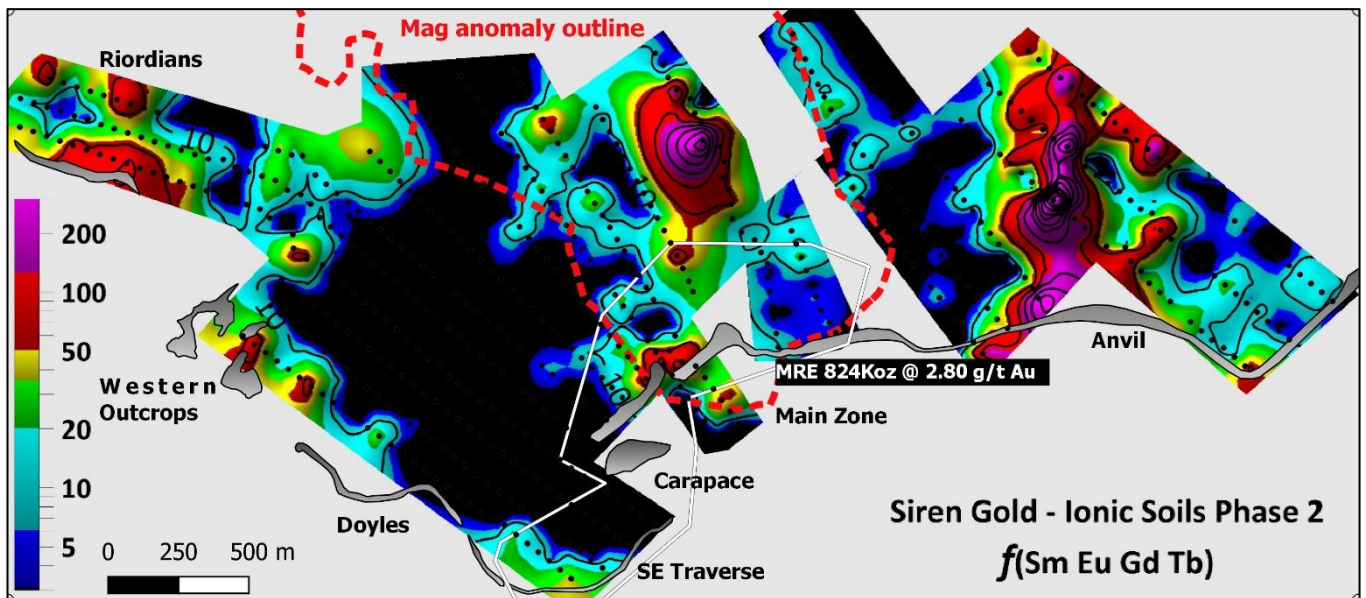
Figure 11. Light REE association (Samarium, Europium, Gadolinium and Terbium)
