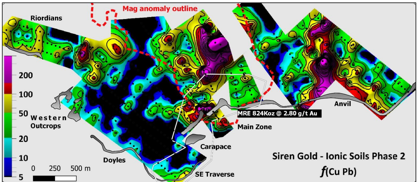
Figure 9. Copper and Lead element association.
