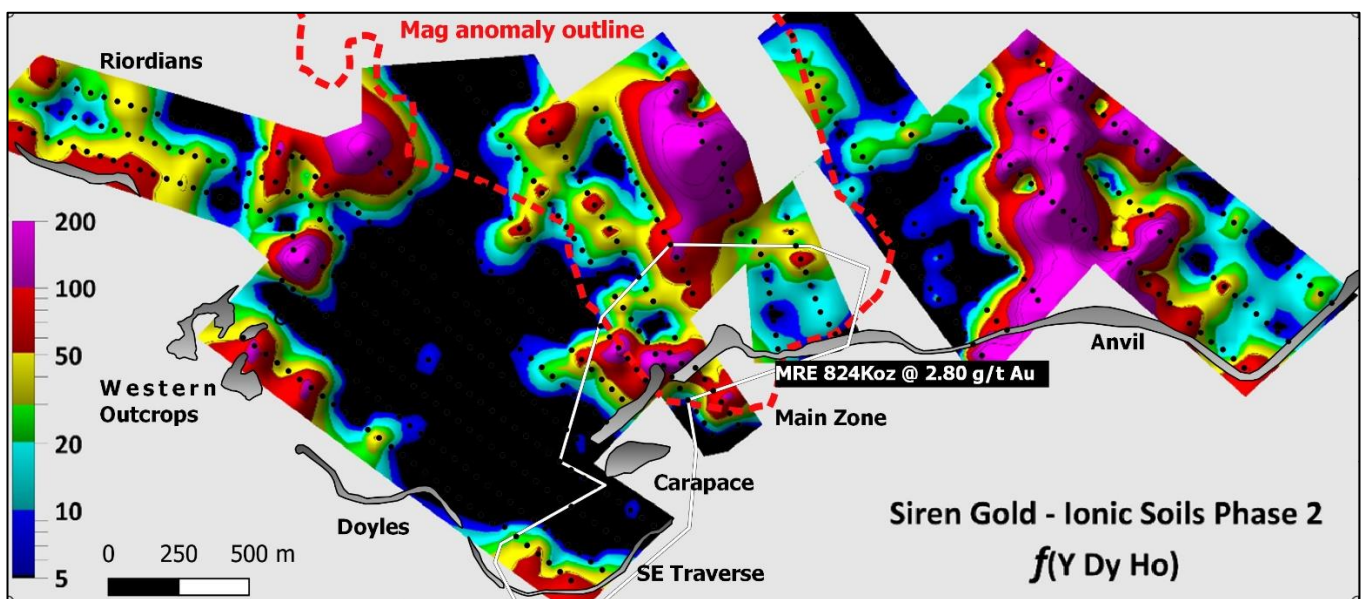
Figure 12. Heavy REE association (Yttrium, Dysprosium, and Holmium)
